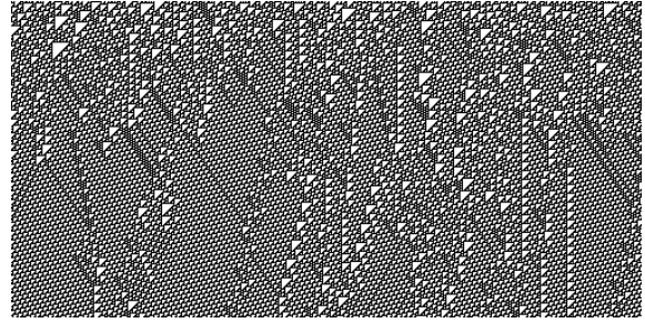
(class 4: rule 110)
