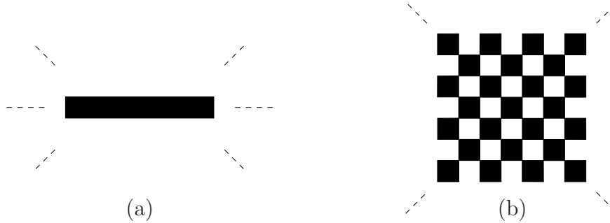
Figure 7: (a) A spatially periodic configuration that is not strongly periodic, and (b) a strongly periodic configuration.
