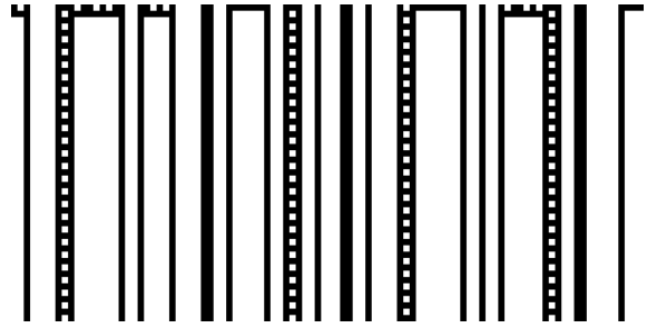
(class 2: rule 108)
