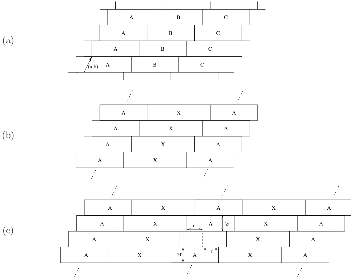
Figure 21: Illustrations for the proof of Proposition 29: (a) Partitioning of the plane into rectangles, (b) an infinite strip S in the direction of the period, and (c) a strongly periodic tiling.
