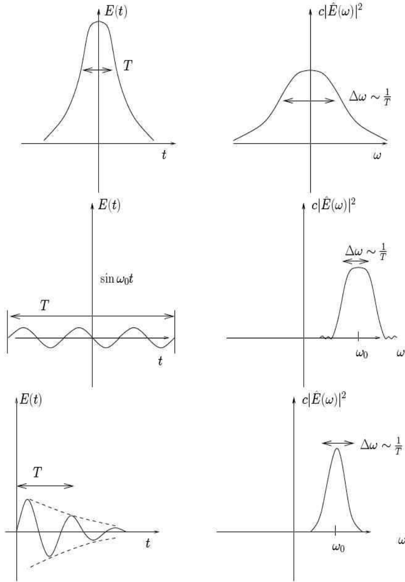
Figure 3.1: EM pulses (left) and associated radiation spectra (right) for three pulse shapes. Top: a pulse of duration T has a spectrum stretching over a bandwidth of \sim 1/T . Middle: A periodic signal with frequency \omega_0 for a total duration of time T will have a spectrum of width \sim 1/T centered on a frequency \omega_0 . Bottom: A similar periodic signal with a decay time of T (damped oscillator) will produce a spectrum of bandwidth \sim 1/T centered on a frequency \omega_0 , but without the higher and lower frequency ‘wiggles’ found in the previous example.
