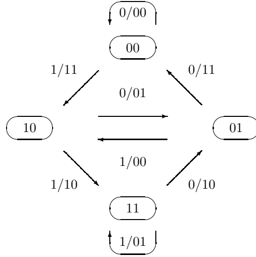
Figure 3.1: State diagram of a (2, 1, 2) encoder of Example 1.3
