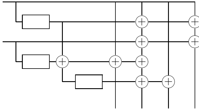
Figure 2.2: Direct-form realization of G_1
