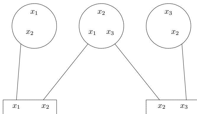
Figure 5.2: An initialization of belief propagation on a Tanner graph
