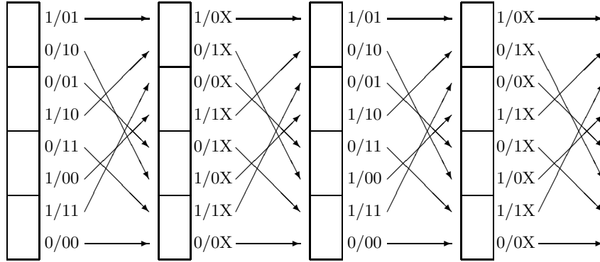
Figure 4.1: A (3, 2, 2) trellis
