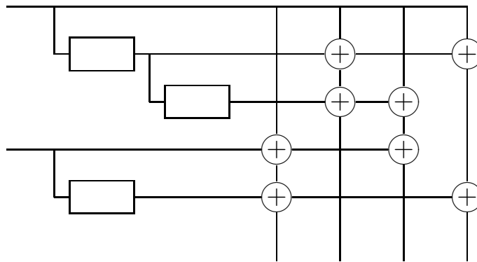
Figure 2.3: Another realization of G_1
